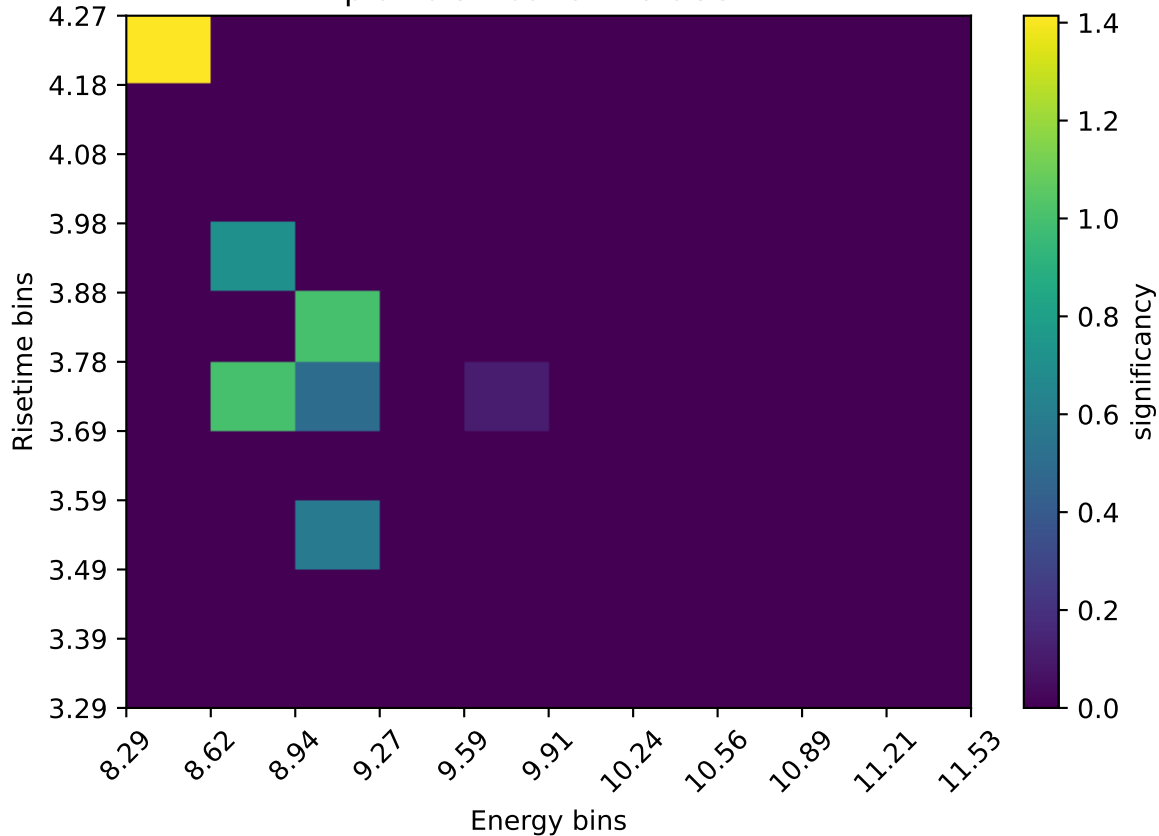
pion distribution 10.0GeV
